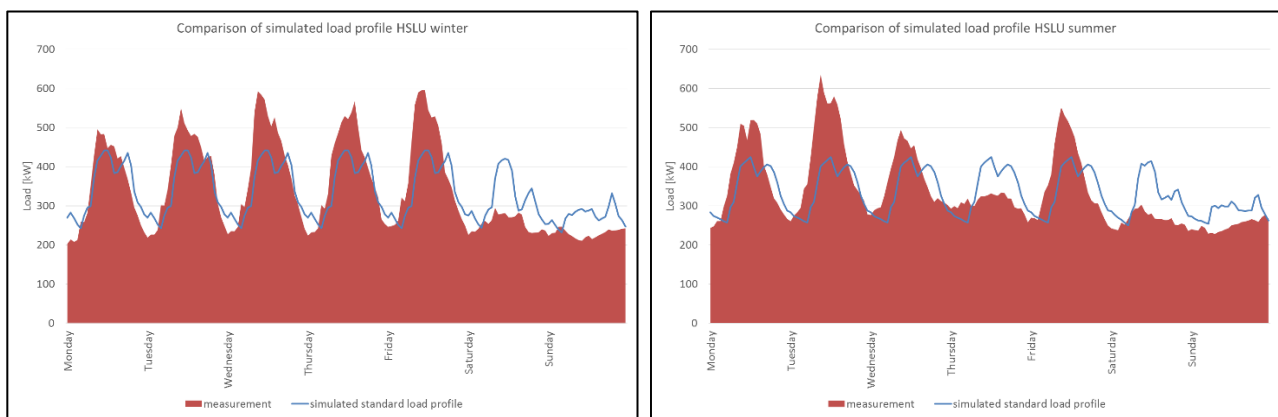
Figure 4: typical weekly winter and summer load profile for office building example measured and simulated
