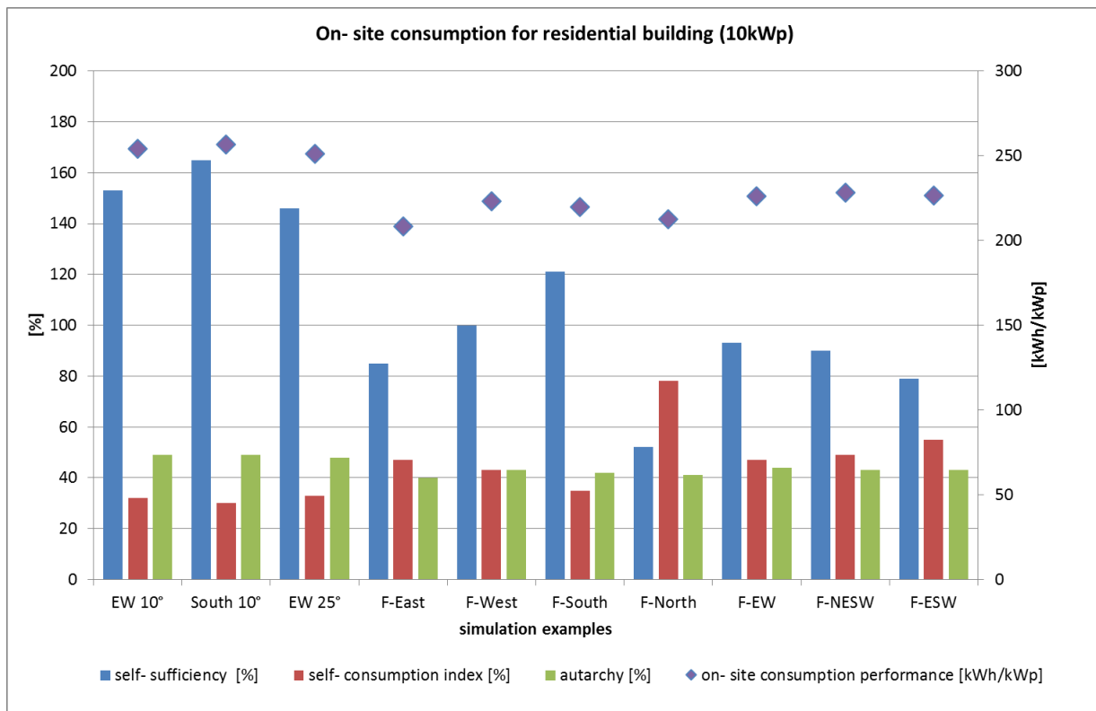
Figure 5: Simulation results for residential building
