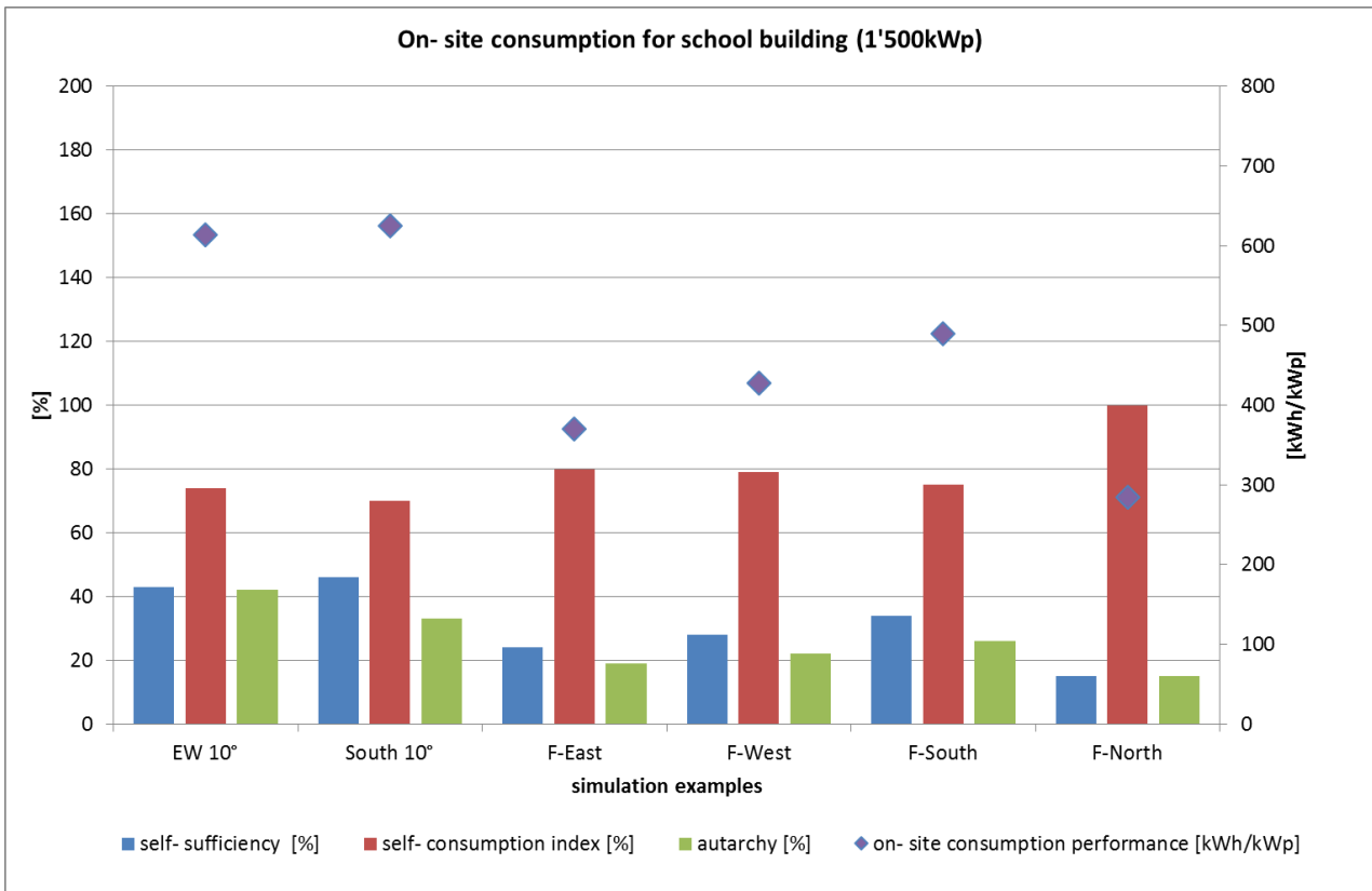
Figure 6: Simulation results for school building
